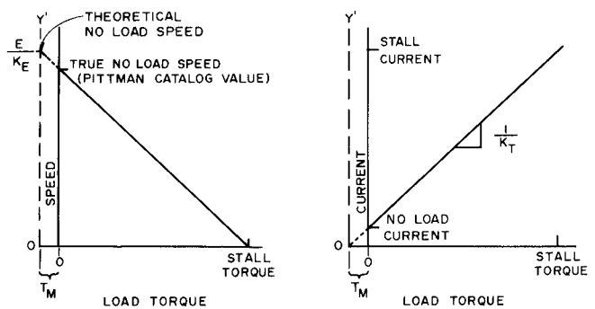
a) Speed vs. Torque b) Current vs. Torque
